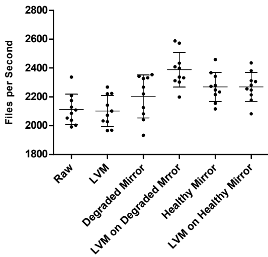
Sequential Read Files Speed
