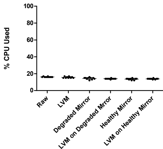
Sequential Delete Files CPU Usage
