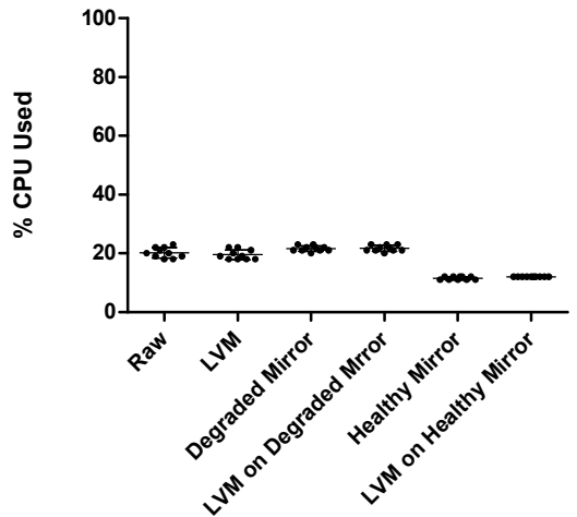
Rewrite Block CPU Usage
