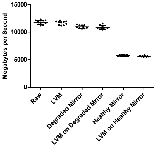
Rewrite Block Speed
