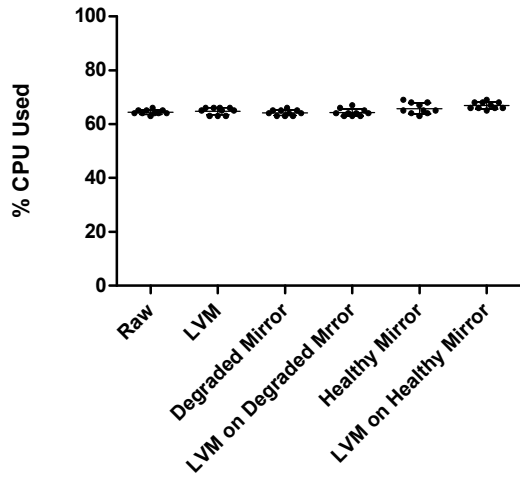
Read Char CPU Usage
