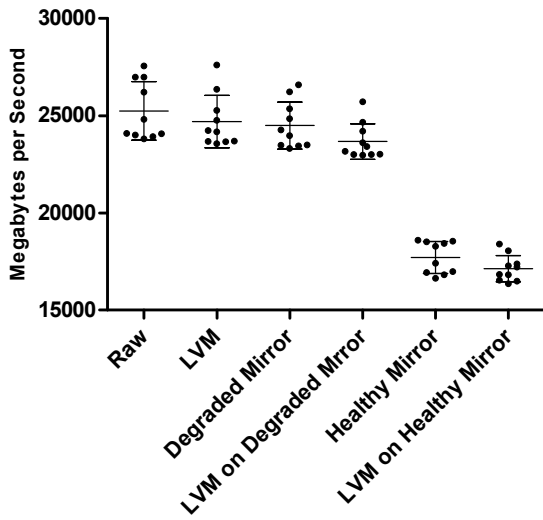
Read Block Speed
