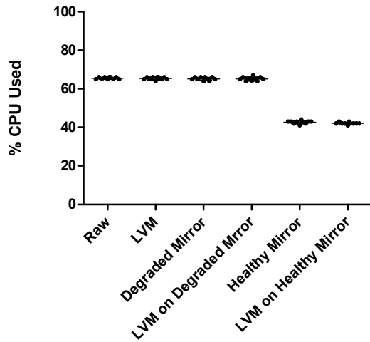
Sequential Create Files CPU Usage
