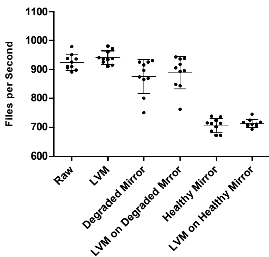
Sequential Delete Files Speed
