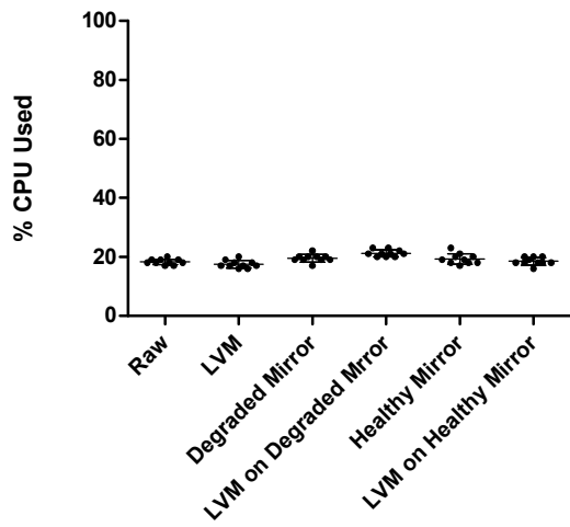
Random Read Files CPU Usage
