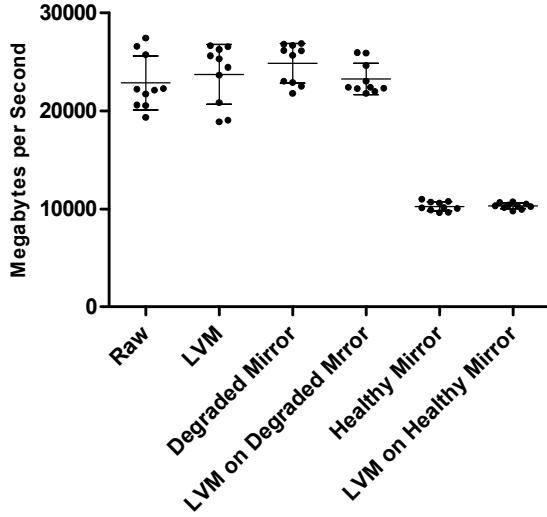
Write Character Speed
