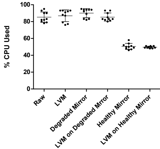
Write Character CPU Usage
