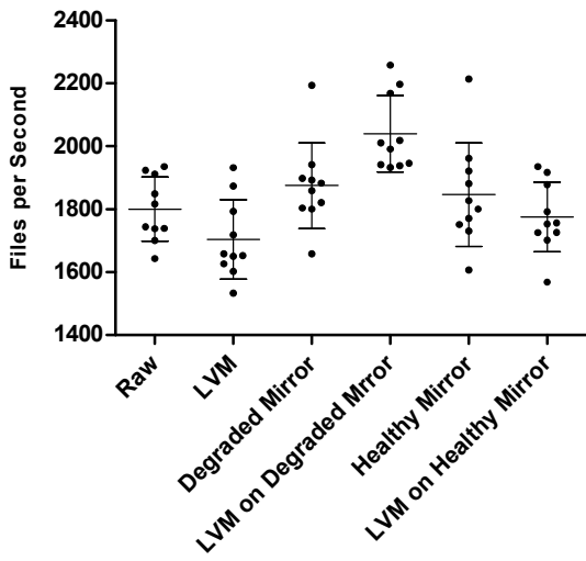
Random Read Files Speed
