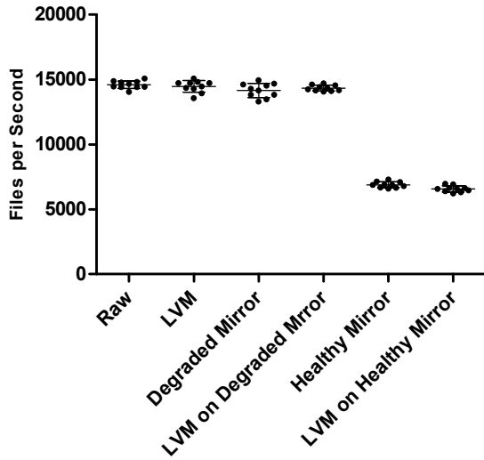
Sequential Create Files Speed
