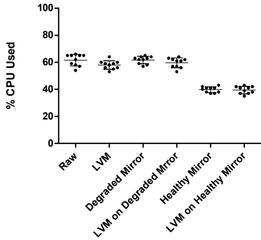
Random Create Files CPU Usage
