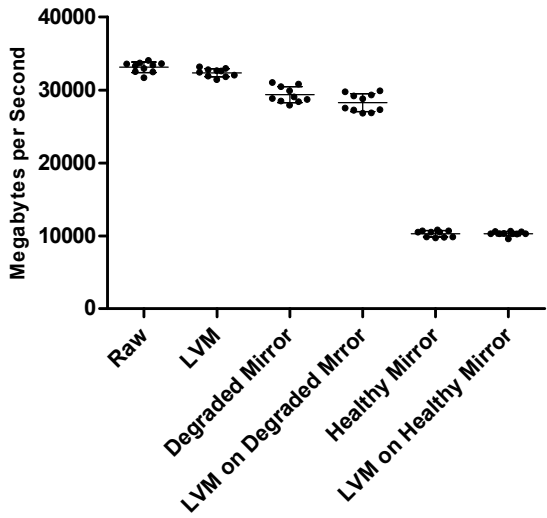
Write Block Speed
